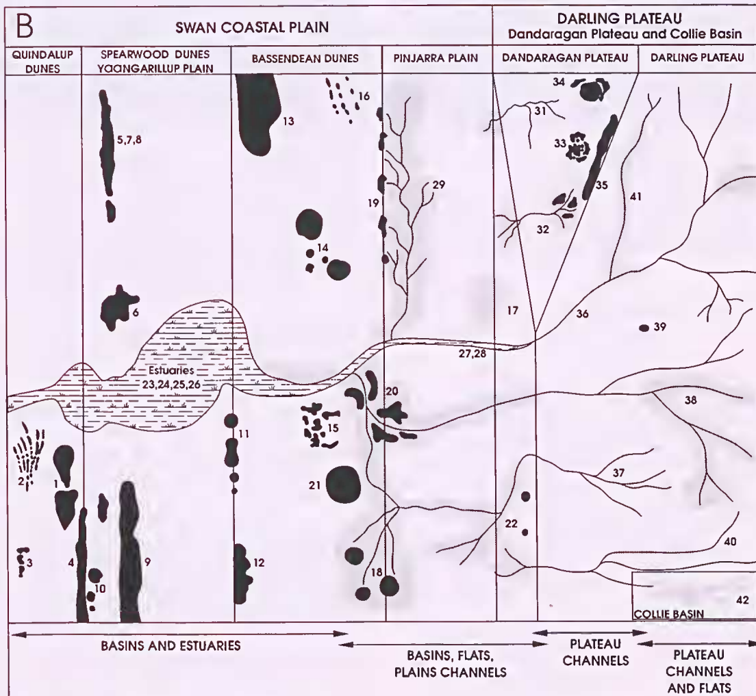
Figure 2. A: Idealised block diagram showing geomorphic units of the Swan Coastal Plain, their sub-parallelism to the Darling Scarp and the coast, their gross surface features, and their stratigraphy, with some details of landscape (after Semeniuk & Glassford 1989). B: Idealised map showing the variety and distribution of consanguineous wetlands (from Semeniuk 1988), i.e., the natural wetland groupings or suites in the Darling Plateau and Swan Coastal Plain centred on the Moore River to Bunbury region. In this region there are 42 such groups each related to geomorphic setting, or interfaces between geomorphic units (for explanation of numbering of the consanguineous wetland suites, see Semeniuk 1988).
